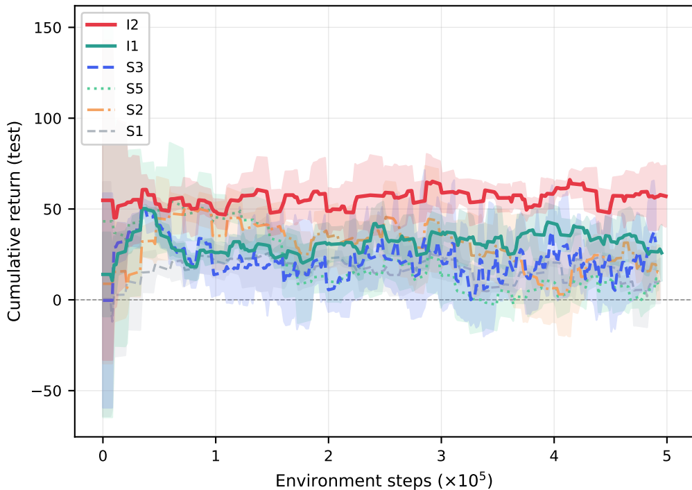
Test return (EWMA-50, mean \pm std)
